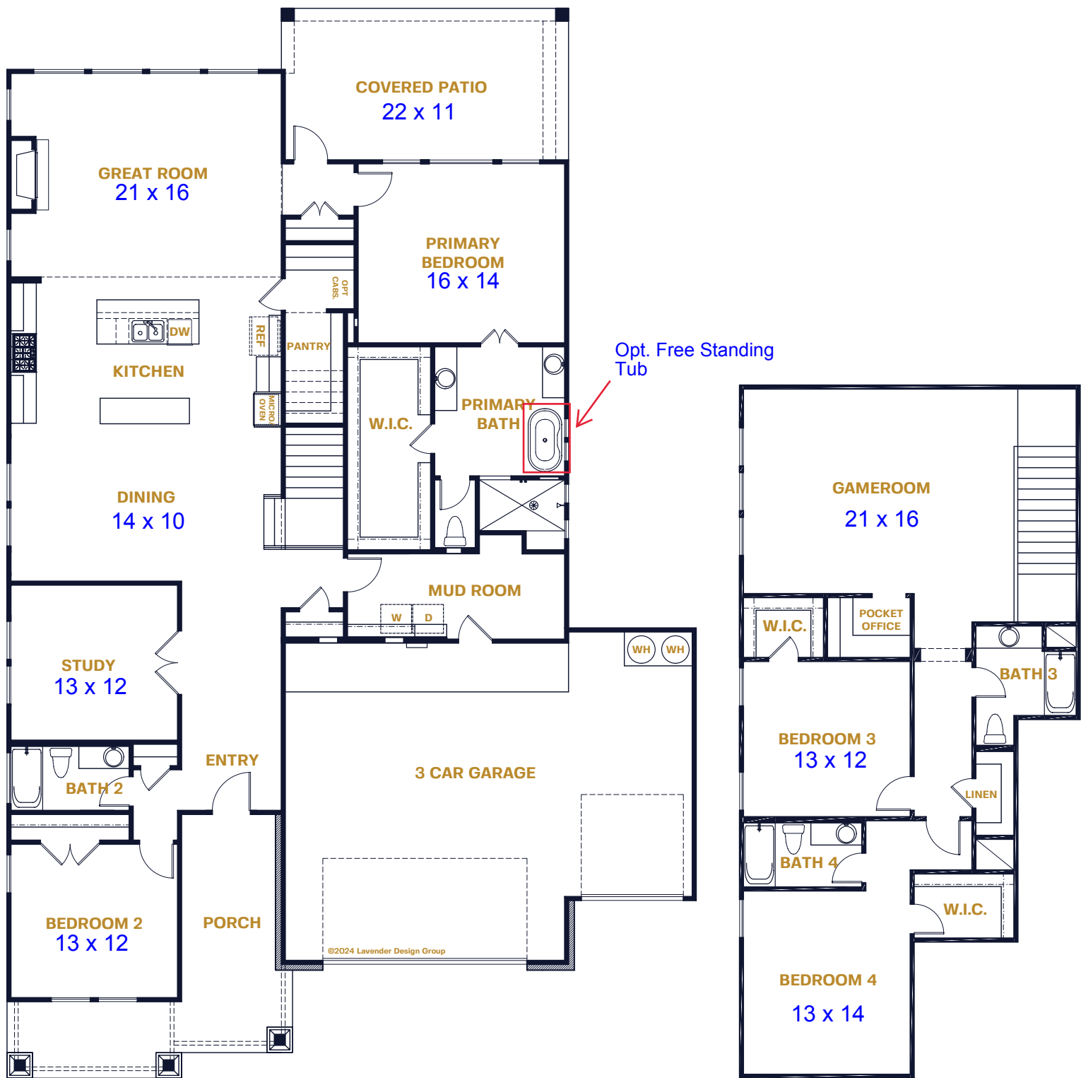
FIRST FLOOR
